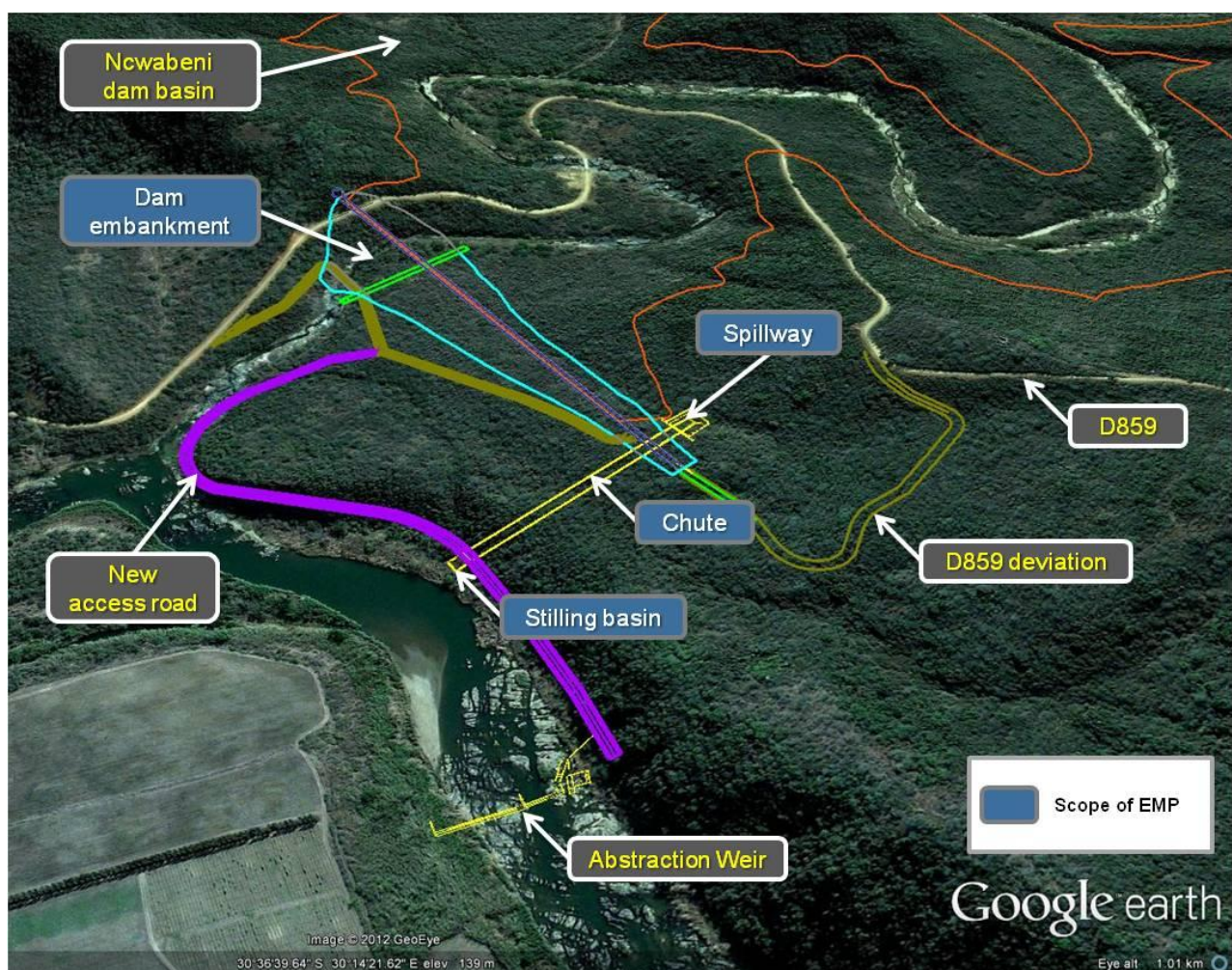
Figure 2: Main Embankment at site D2 (Google Earth image)
