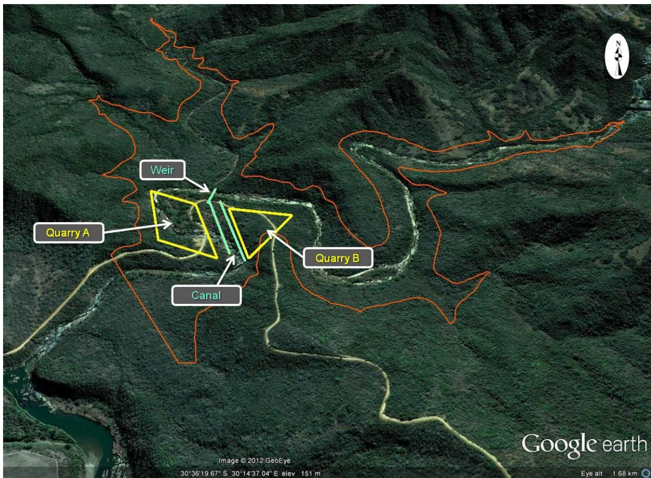
Figure 3: Quarry Areas and River Diversion at site D2 (Google Earth image)
