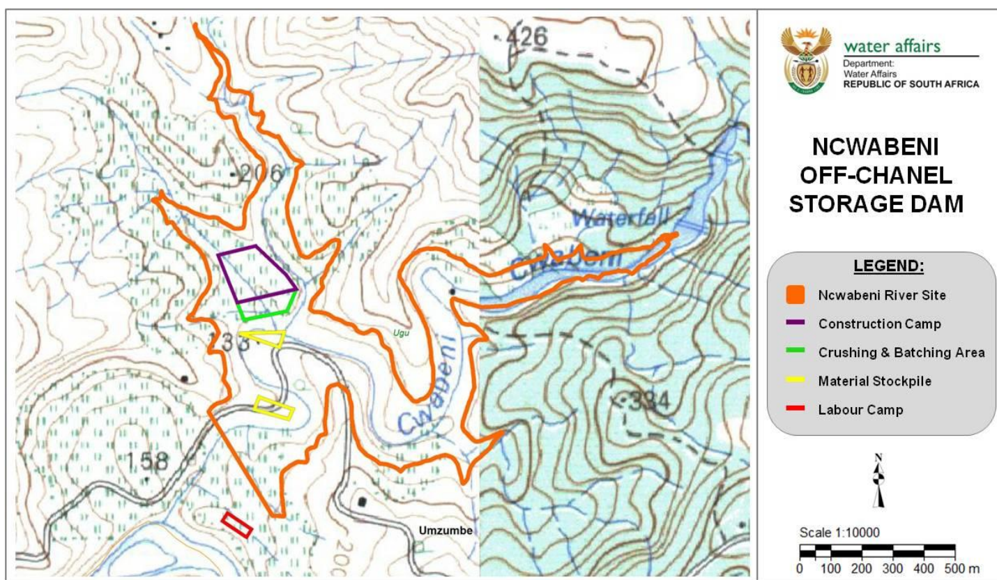
Figure 4: Construction and Labour Camps (and other major construction facilities)
